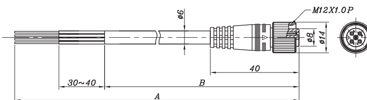
SW-4119 / Plug Connector
